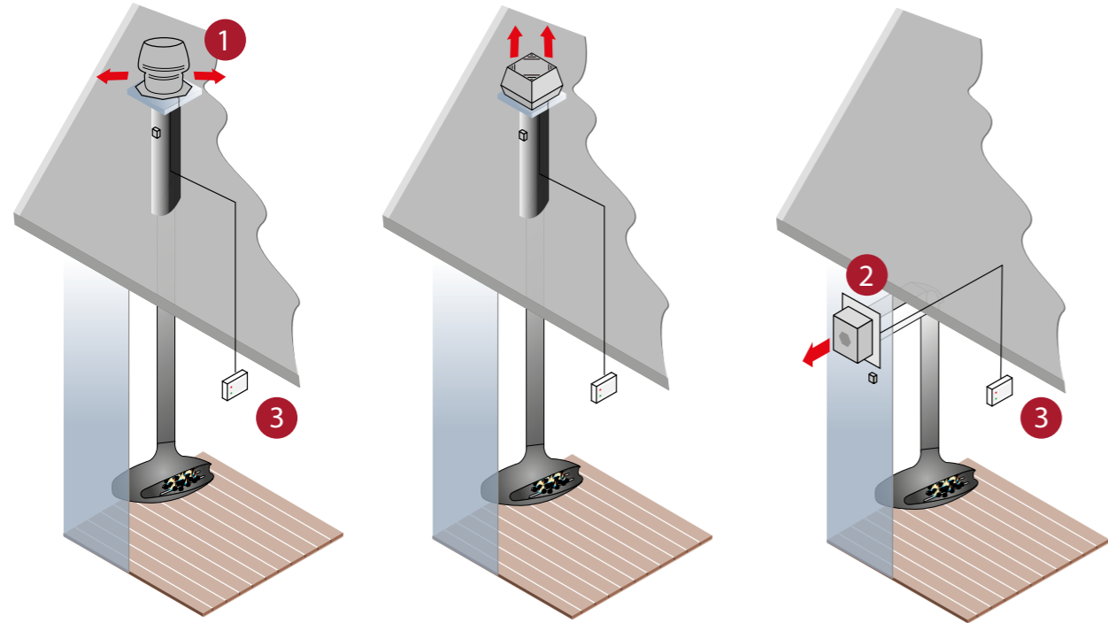
Chimney fan system with horizontal extraction via a steel chimney
